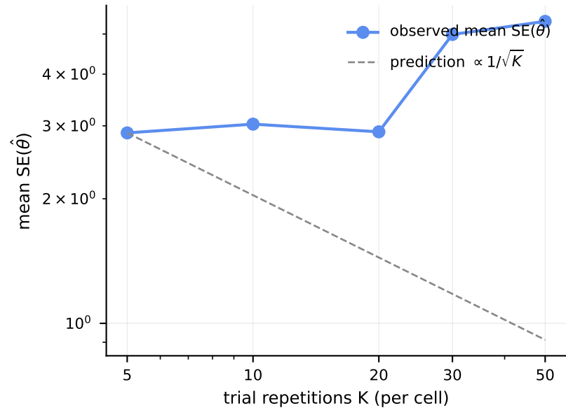
(c) Decision study: K vs SE(\hat{\theta})
