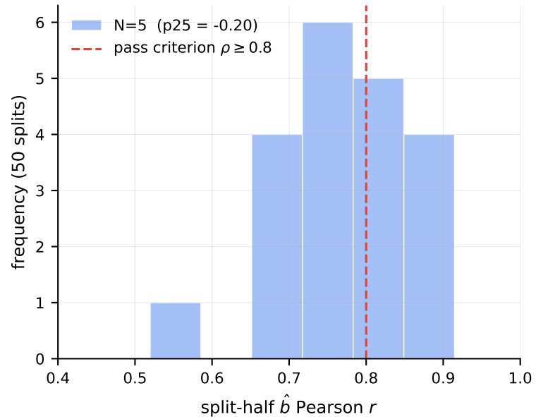
(a) Sample invariance of \hat{b} across AV subsets
