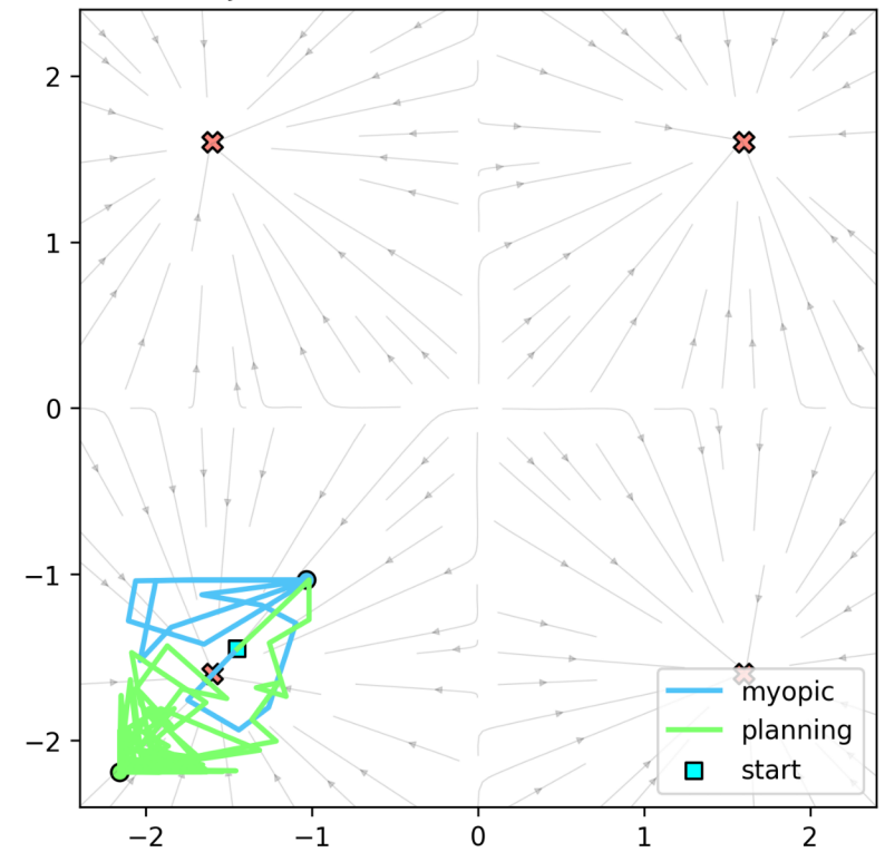
Trajectories on multistable latent field
