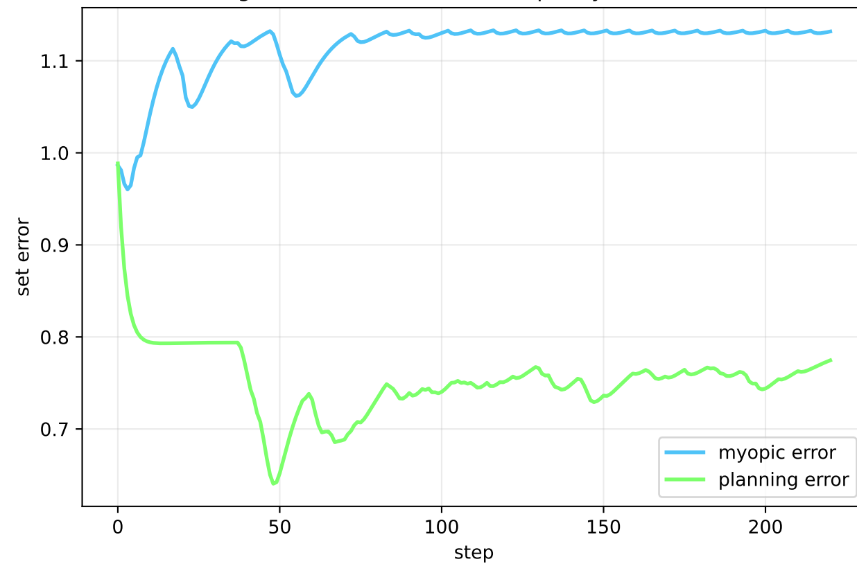
Convergence: attractor estimate quality (lower is better)
