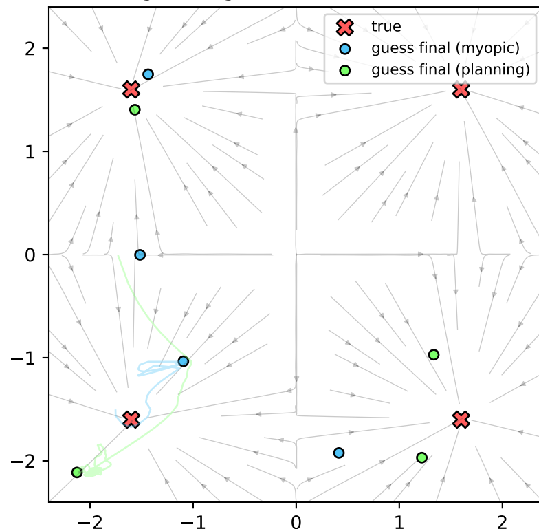
Acquisition behavior over time
