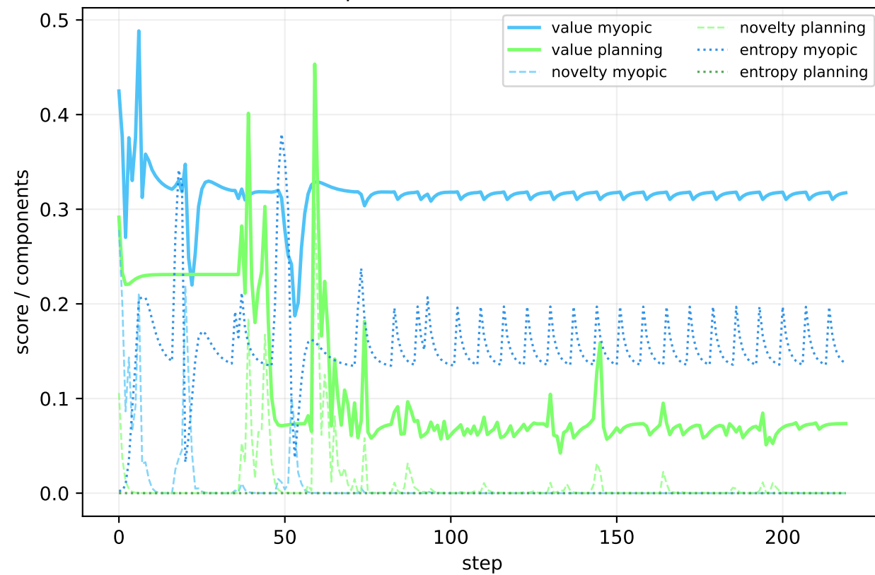
Acquisition behavior over time
