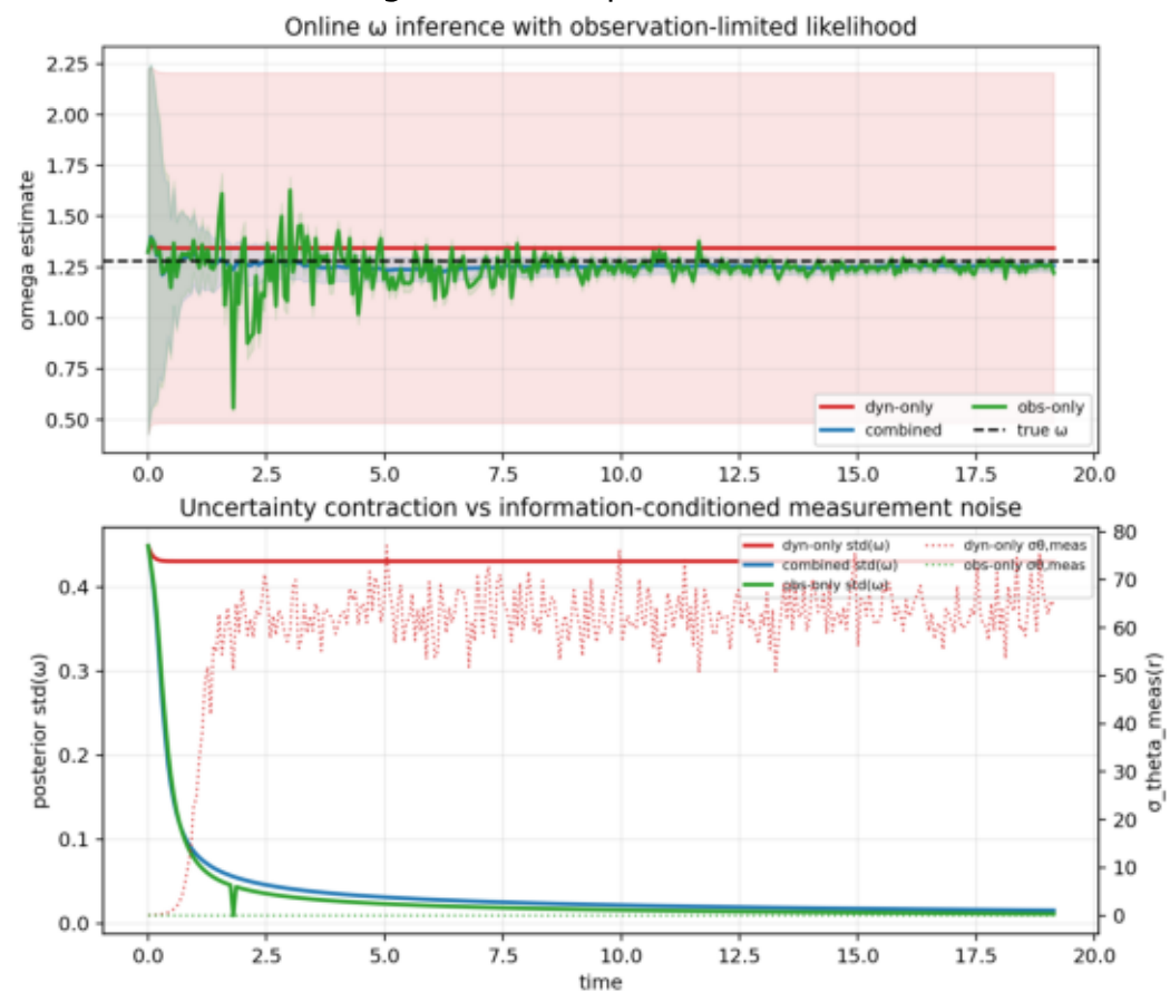
(C) omega estimate/posterior evolution
