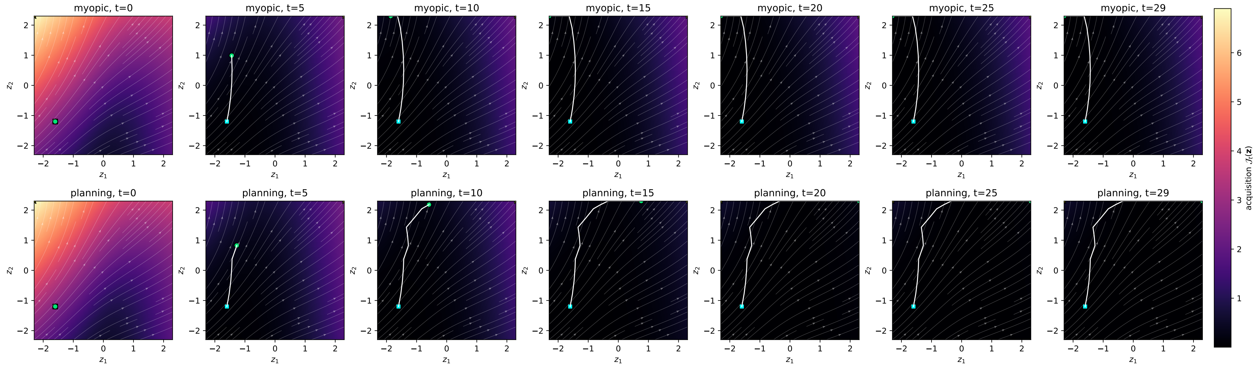
Time-resolved acquisition evolution: myopic vs planning-based active learning
