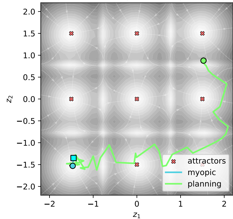
Underlying multistable dynamics + policy trajectories
