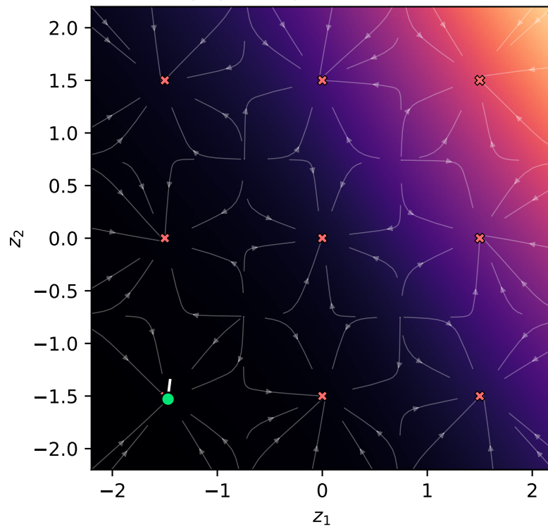
Myopic acquisition at t=21
