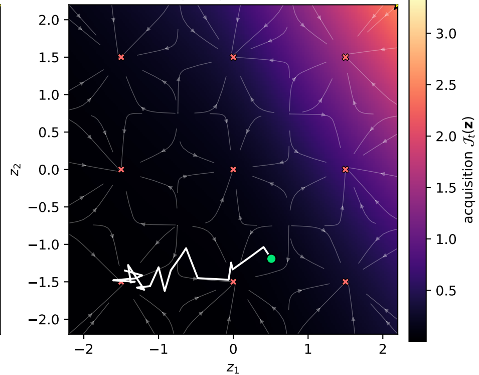
Planning acquisition at t=21
