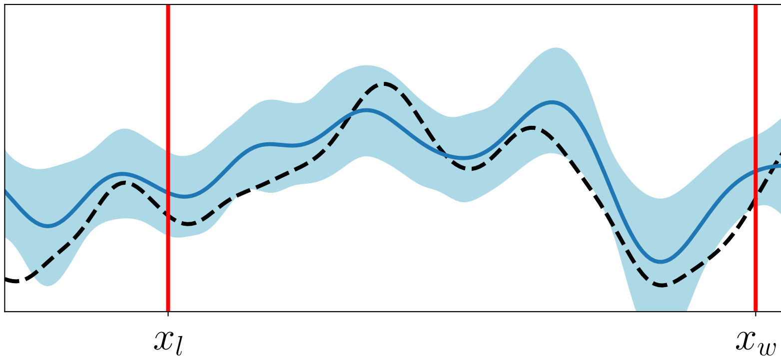
MCMC
