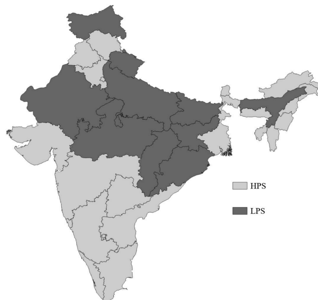
Figure 1: Low- and High-Performing States under the JSY Program
