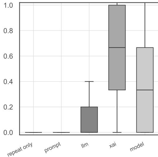
Rank distance
