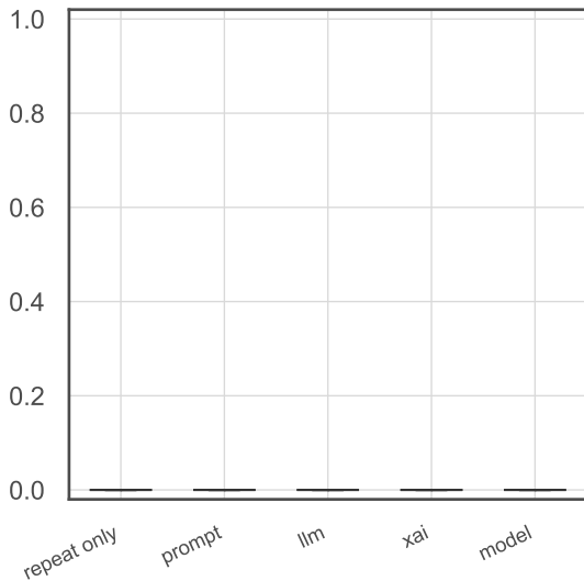
Direction distance
