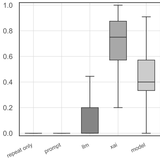
Feature distance
