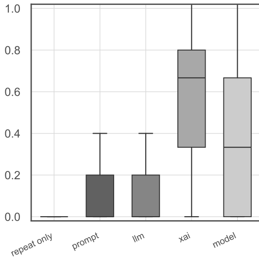
Rank distance
