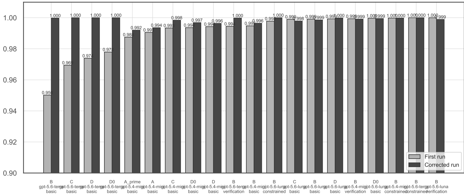
Direction agreement
