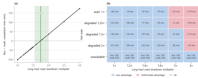
FIGURE 6. Fixed-12/11-split road–rail decision boundary (top-10, reverse empty return, 30 CRN seeds). (a) Mean completion-time difference versus long-haul road multiplier with normally available rail; interpolated crossing 1.742 with joint-seed bootstrap 95% interval 1.550–2.003. (b) Technical winner across road slowdown and rail-state combinations; cells with both alternatives complete show time difference, rail-unavailable cells show completion rates. The crossing is conditional on the stated demand, resource frame, rail state, and the fixed 12/11 fleet split; the allocation-dependent band is reported in Table 12.
