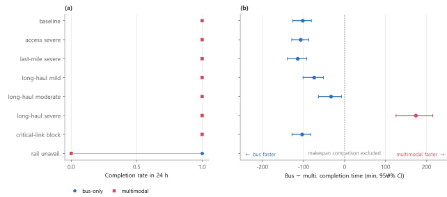
FIGURE 4. Equal-road-fleet paired stress comparison at the fixed 12/11 split (top-10, reverse empty return, 30 CRN seeds; road-vehicle totals matched, rail cost not matched). (a) Completion rate within 24 h; (b) mean completion-time difference \Delta = bus-only - static multimodal with percentile-bootstrap 95% intervals. Negative values favor bus-only; positive values favor multimodal. Only the extreme long-haul damage cell flips the time ordering; rail-unavailable cells are ranked on completion rate only. Allocation-conditional baselines are reported in Table 6.
