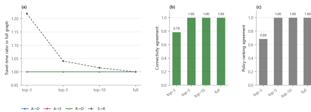
FIGURE 3. Reduced-graph scope sensitivity. (a) Functional-segment travel-time ratios of top-3, top-5, and top-10 envelopes versus the full reference graph; (b) connectivity agreement (70 outcomes) and (c) bus-static policy-ranking agreement (35 comparisons) under seven configured-bundle scenarios and five common seeds. Top-5 and top-10 equal 1.00 on both agreements; top-3 is 0.786 and 0.686. S \rightarrow R normal-time ratios are 1.218 (top-3) and 1.015 (top-10). Results hold only for the tested conditions.
