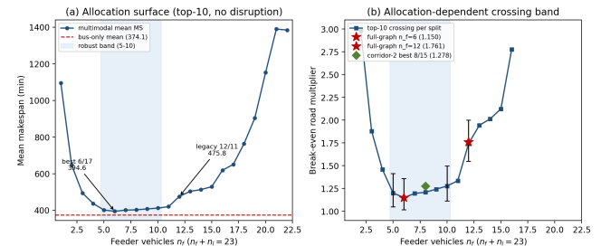
FIGURE 5. Allocation-conditional boundary (top-10, matched road fleet, available rail, 30 seeds). (a) Mean multimodal makespan across all 23 feasible feeder/last-mile splits at no disruption; dashed line is the bus-only mean (374.1 min) and shading marks the robust band (splits 5–10). (b) Break-even crossing per split with joint-seed 95% intervals at splits 5, 6, 10, and 12; red stars are full-graph validation points and the green diamond is the second-corridor crossing at its own best split. The crossing sweeps from about 1.15 to 2.78 across feasible splits.
