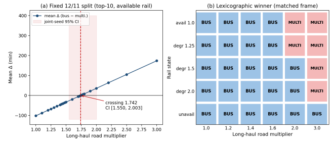
FIGURE 6. Fixed-12/11-split road-rail decision boundary (top-10, reverse empty return, 30 CRN seeds). (a) Mean completion-time difference versus long-haul road multiplier with normally available rail; interpolated crossing 1.742 with joint-seed bootstrap 95% interval 1.550–2.003. (b) Technical winner across road slowdown and rail-state combinations; cells with both alternatives complete show time difference, rail-unavailable cells show completion rates. The crossing is conditional on the stated demand, resource frame, rail state, and the fixed 12/11 fleet split; the allocation-dependent band is reported in Table 14.
