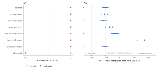
FIGURE 4. Equal-road-fleet paired stress comparison at the fixed 12/11 split (top-10, reverse empty return, 30 CRN seeds; road-vehicle totals matched, rail cost not matched). (a) Completion rate within 24 h; (b) mean completion-time difference \Delta = bus-only – static multimodal with percentile-bootstrap 95% intervals. Negative values favor bus-only; positive values favor multimodal. Only the extreme long-haul damage cell flips the time ordering; rail-unavailable cells are ranked on completion rate only. Allocation-conditional baselines are reported in Table 7.
