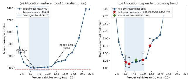
FIGURE 5. Allocation-conditional boundary (top-10, matched road fleet, available rail, 30 seeds). (a) Mean multimodal makespan across all 22 feasible feeder/last-mile splits at no disruption; dashed line is the bus-only mean (374.1 min) and shading marks the 5%-regret band (splits 5–10). (b) Break-even crossing per split with joint-seed 95% intervals at splits 5, 6, 10, and 12; red stars are full-graph validation points and the green diamond is the second-corridor crossing at its own best split. The crossing sweeps from about 1.15 to 2.78 across feasible splits.
