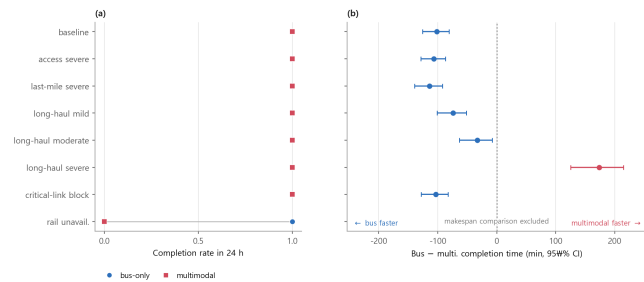
FIGURE 4. Equal-road-fleet paired stress comparison (top-10, reverse empty return, 30 CRN seeds; road-vehicle totals matched, rail cost not matched). (a) Completion rate within 24 h; (b) mean completion-time difference \Delta = bus-only - static multimodal with percentile-bootstrap 95% intervals. Negative values favor bus-only; positive values favor multimodal. Only the extreme long-haul damage cell flips the time ordering; rail-unavailable cells are ranked on completion rate only.
