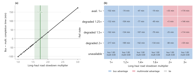
FIGURE 5. Equal-road-fleet road-rail decision boundary (top-10, reverse empty return, 30 CRN seeds). (a) Mean completion-time difference versus long-haul road multiplier with normally available rail; interpolated crossing 1.742 with joint-seed bootstrap 95% interval 1.550–2.003. (b) Technical winner across road slowdown and rail-state combinations; cells with both alternatives complete show time difference, rail-unavailable cells show completion rates. The crossing is a conditional boundary for the stated demand, resource frame, and rail state.
