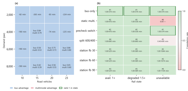
FIGURE 6. Fleet scarcity and rail-state response policies (top-10, reverse empty return, 30 CRN seeds). (a) Outcome-winner map over demand (2,000–8,000 passengers) and equal total road-fleet size (10–23 vehicles) with available rail and no road damage; cell color is the lexicographic winner (blue bus-only, red multimodal, gray tie) and annotations give completion rates (bus/multi.) where they differ and mean \Delta in minutes where both complete. Bus-only wins or ties every cell; higher-demand cells separate on completion rate rather than makespan. (b) Policy ranking at demand 1,000 and 23 road vehicles under completion-rate-then-makespan ordering; when rail is unavailable, precheck switching ties bus-only while static multimodal has completion 0.00.
