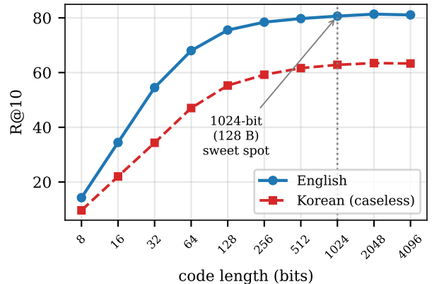
Figure 2: Bit-rate sweep, COCO (lowercased). 1024-bit (128 B) is the deployed sweet spot; 2048-bit adds +0.7 R@10 for 2× storage. Source: paper/bits_extreme_lc.csv.
