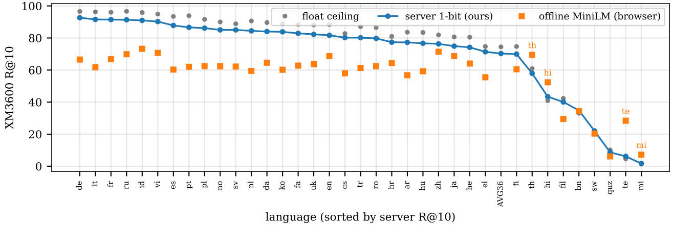
Figure 3: XM3600 per-language R@10 (36 languages, sorted by server score): float ceiling, our 1-bit server path, and the offline browser encoder. On four low-resource non-Latin languages (hi, te, th, mi) the offline encoder beats the server path—the text tower, not binarization, is the bottleneck there. Source: paper/multiling_server_lc.csv.
