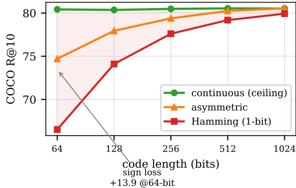
Figure 4: Continuous vs. Hamming vs. asymmetric R@10 by bit length (nested head, ceiling path). The shaded band is the sign loss; it is large at 64-bit and vanishes by 1024-bit, and asymmetric search recovers about half of it. Source: paper/signloss_quant.csv.
