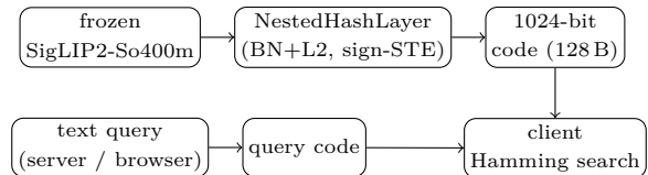
Figure 1: System architecture. Gallery codes (top) are precomputed once; queries (bottom) are encoded by one of two text paths (§2.2) and matched by client-side Hamming distance. No retrieval backend.
