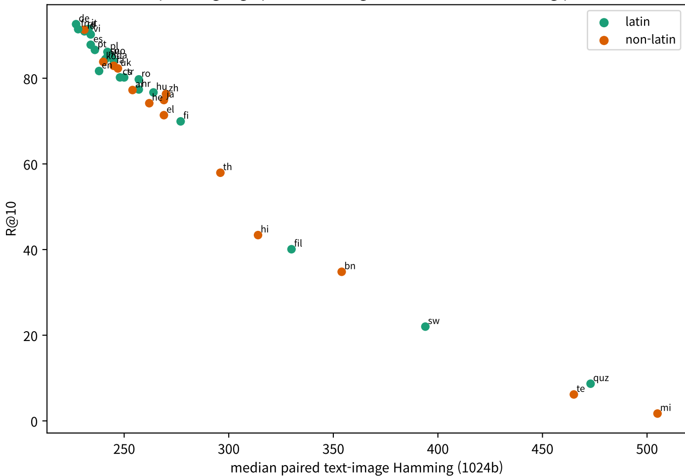
E1: per-language pair-Hamming vs R@10 (XM3600, ceiling path)
