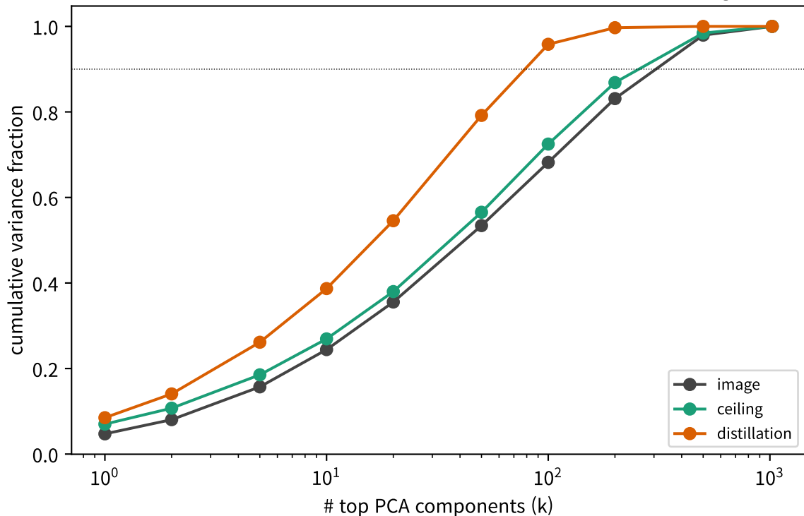
F1: cumulative explained variance (backbone embeddings)
