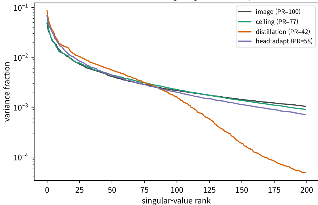
A1: backbone embedding singular-value spectrum
