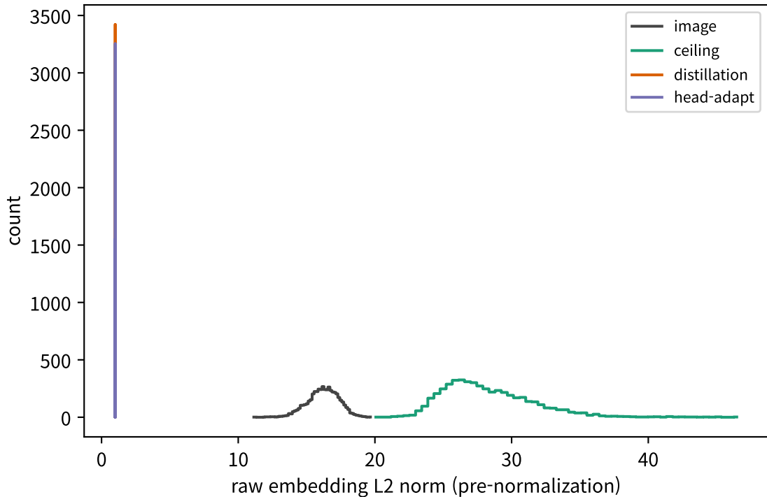
A3: raw embedding norm distribution
