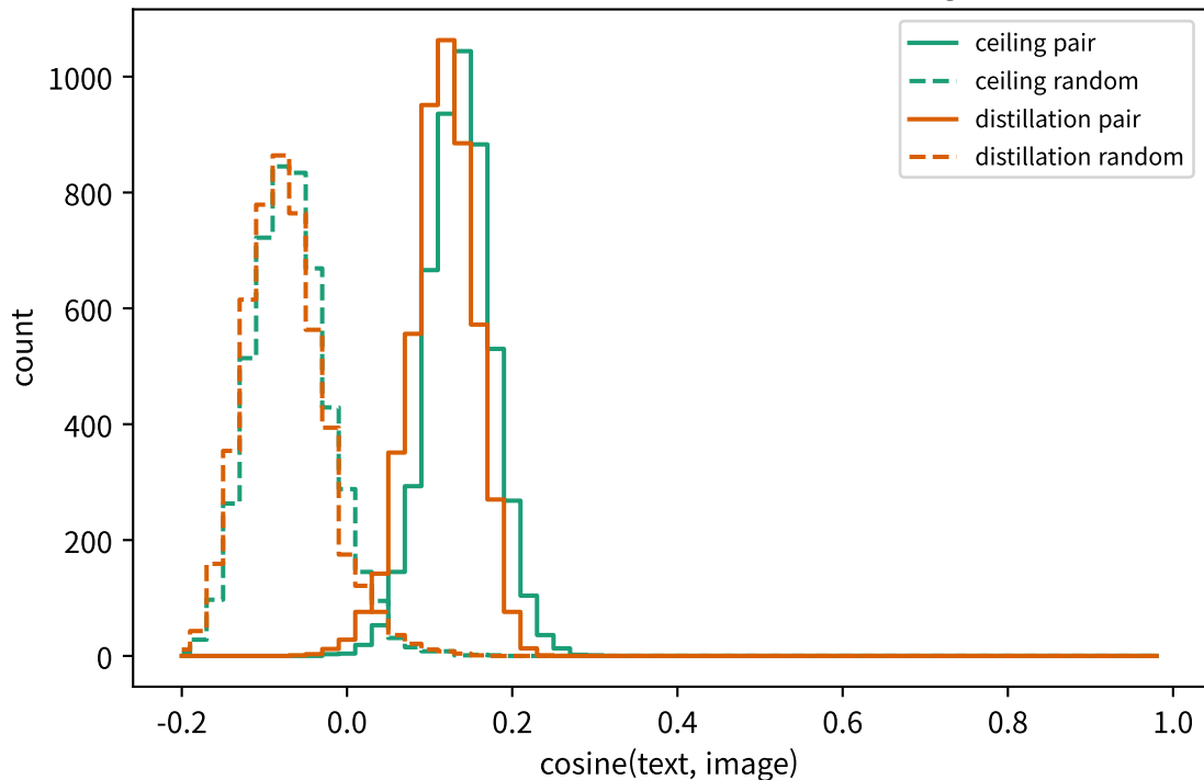
A4: paired vs random cross-modal cosine (SigLIP space)
