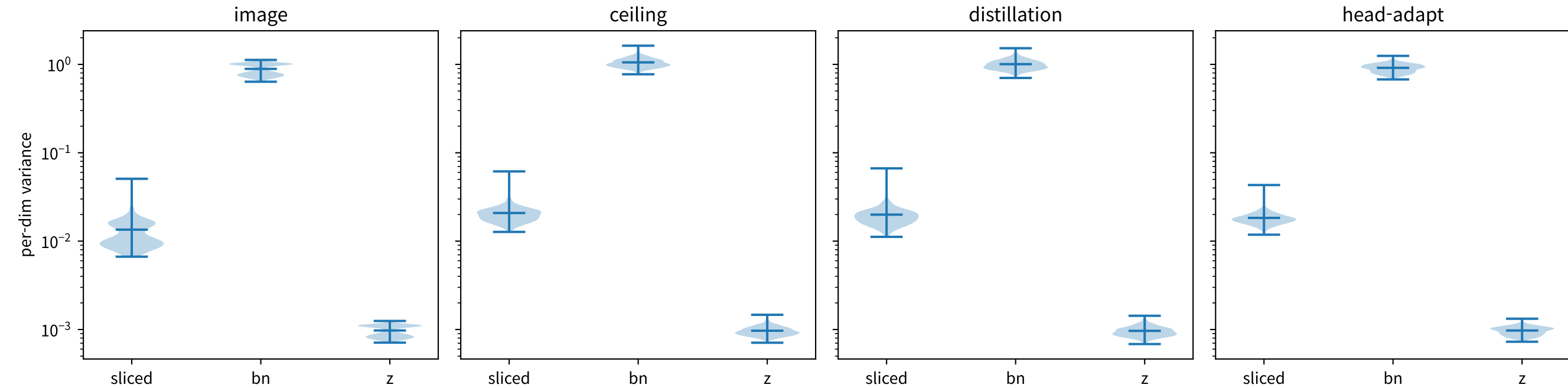
B1: per-dim variance by head stage (sliced -> BN -> L2 z)
