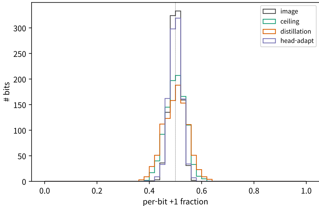
C1: per-bit activation balance (1024 bits)
