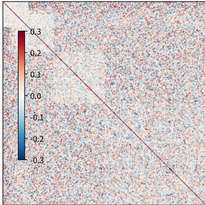
head-adapt
