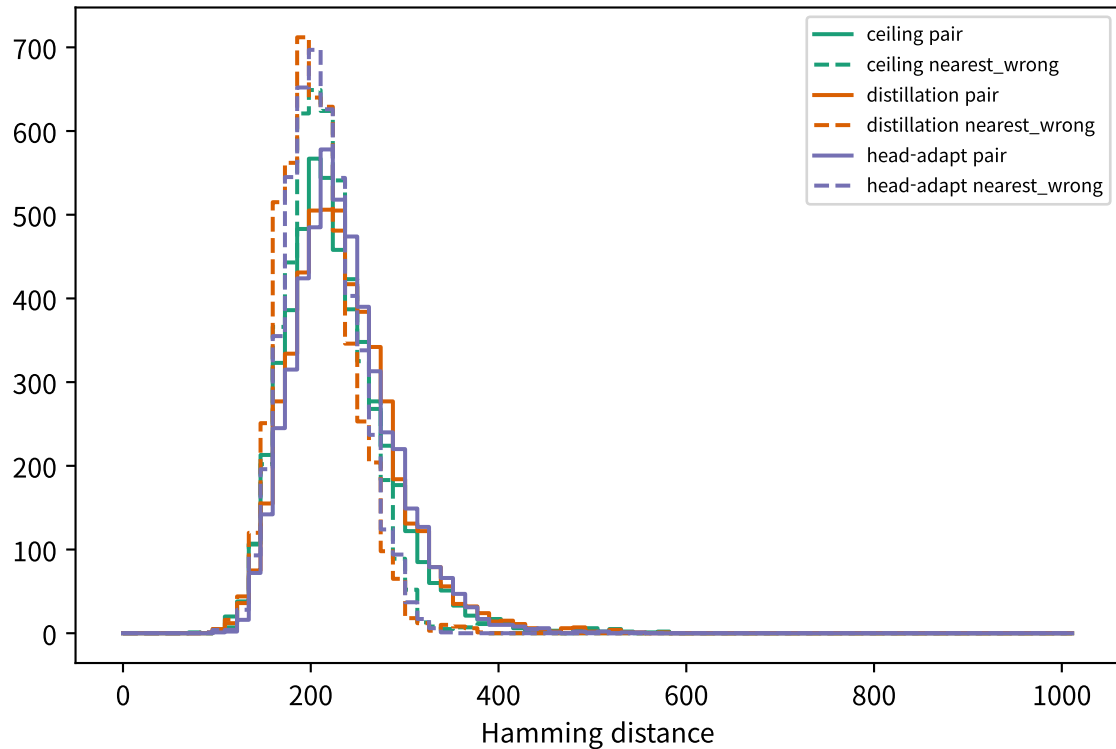
C3: pair vs nearest-wrong Hamming (1024b)
