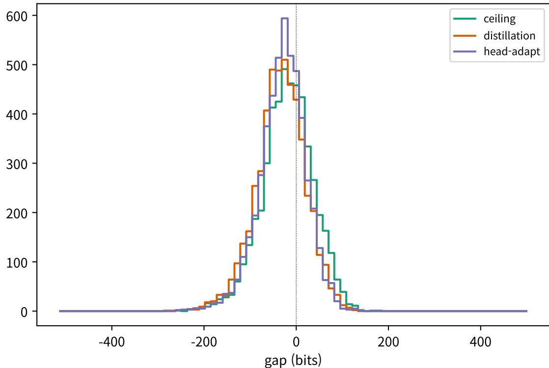
C3: separation gap (nearest_wrong - pair)
