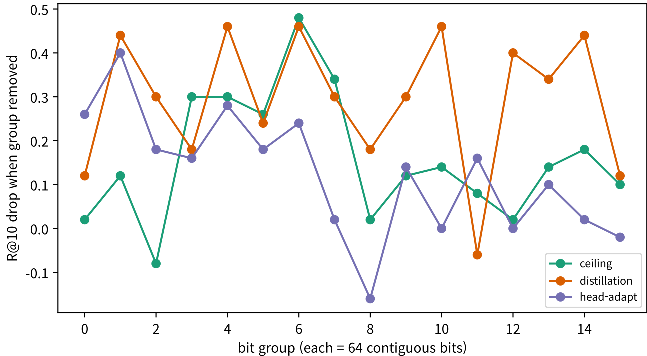
C4: grouped bit-ablation contribution
