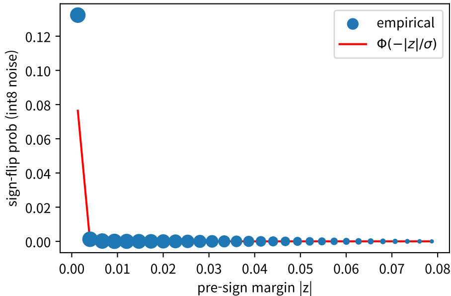
flip vs margin (weighted R^2=0.81 )
