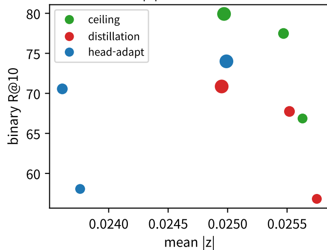
mean|z| vs R@10 (-0.30)
