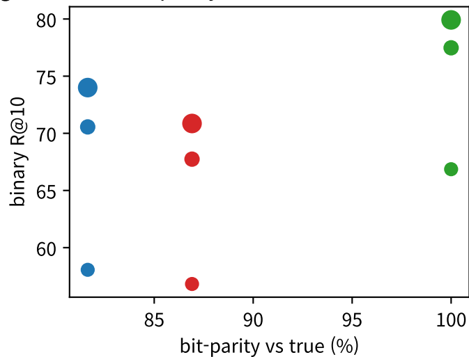
parity vs R@10 (0.32)
