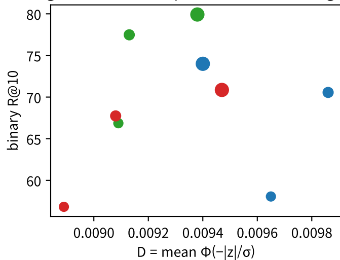
margin D vs R@10 (Spearman 0.25, wrong sign)
