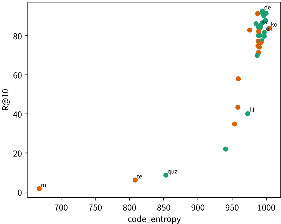
code dir-align (proxy; pair-Hamming = tautology) Spearman \rho = +0.980
