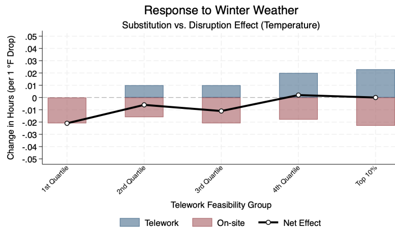
(b) Temperature
