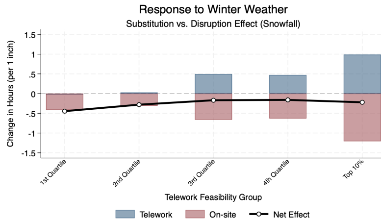
(a) Snowfall
