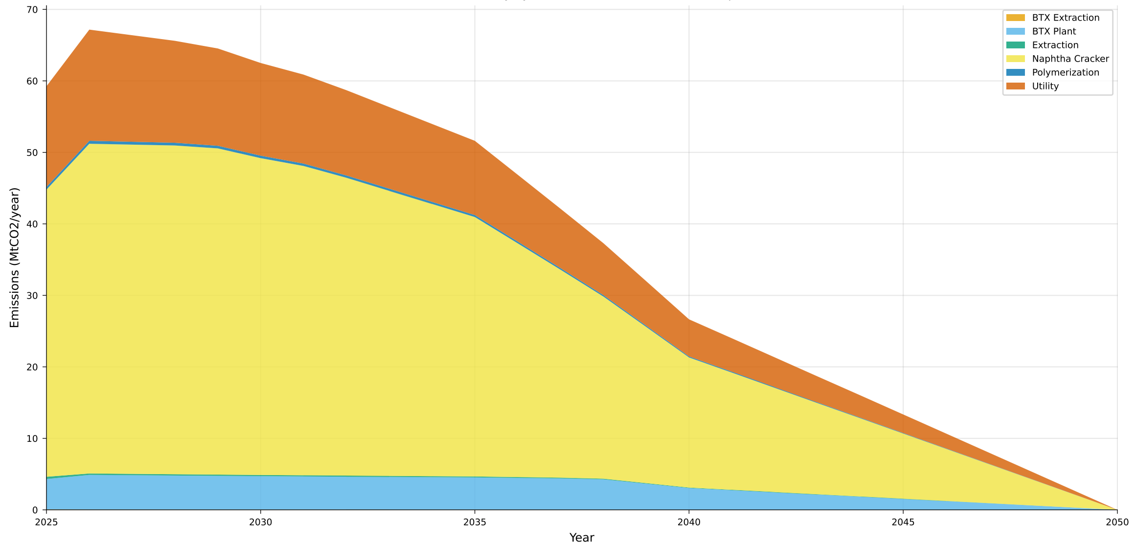
Emission Pathway by Process - NCC-Elec (Flat + Decoupled)
