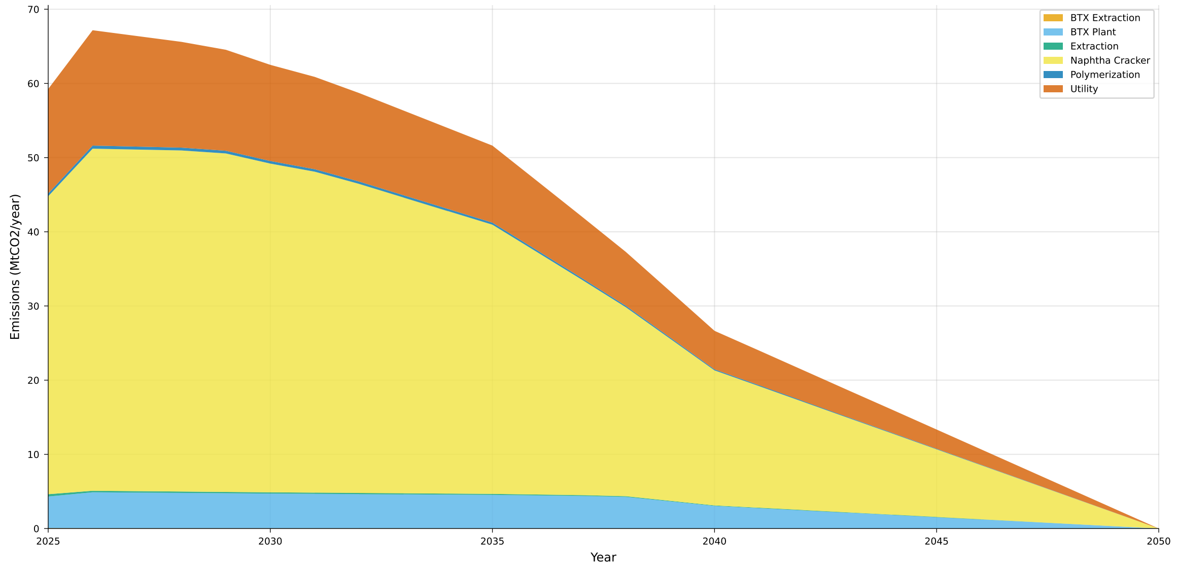
Emission Pathway by Process - NCC-Elec (Rising + Coupled)
