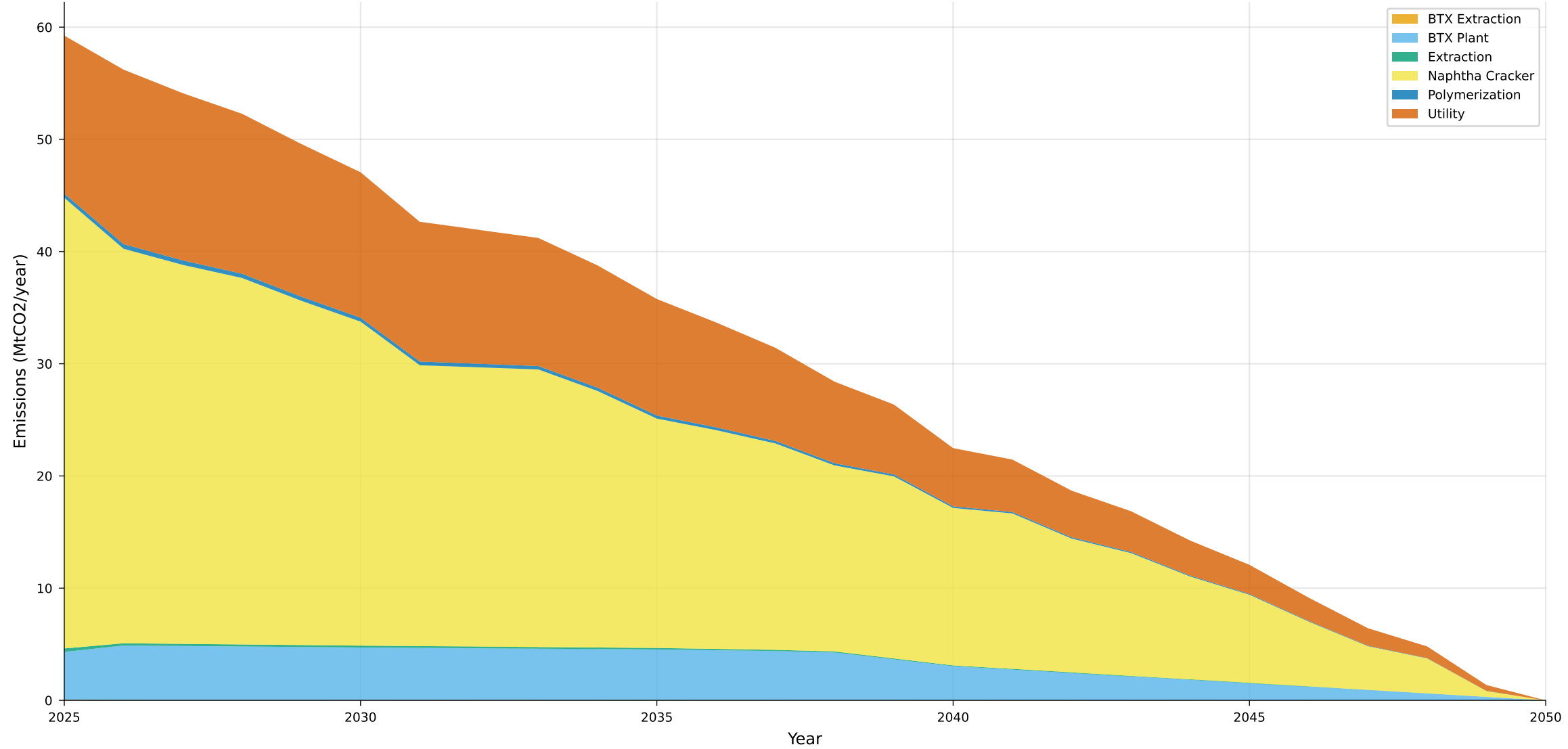
Emission Pathway by Process - NCC-H2 (Flat + Coupled)
