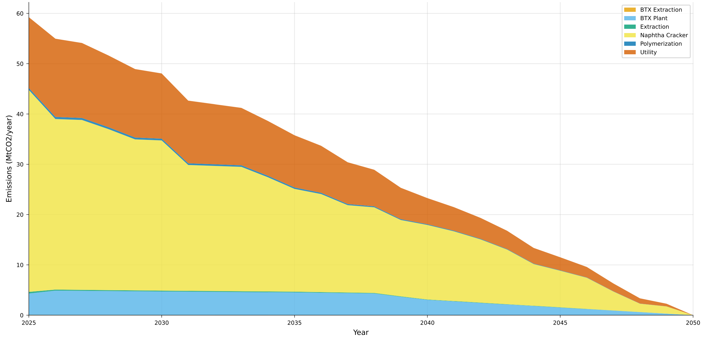
Emission Pathway by Process - NCC-H2 (Rising + Coupled)
