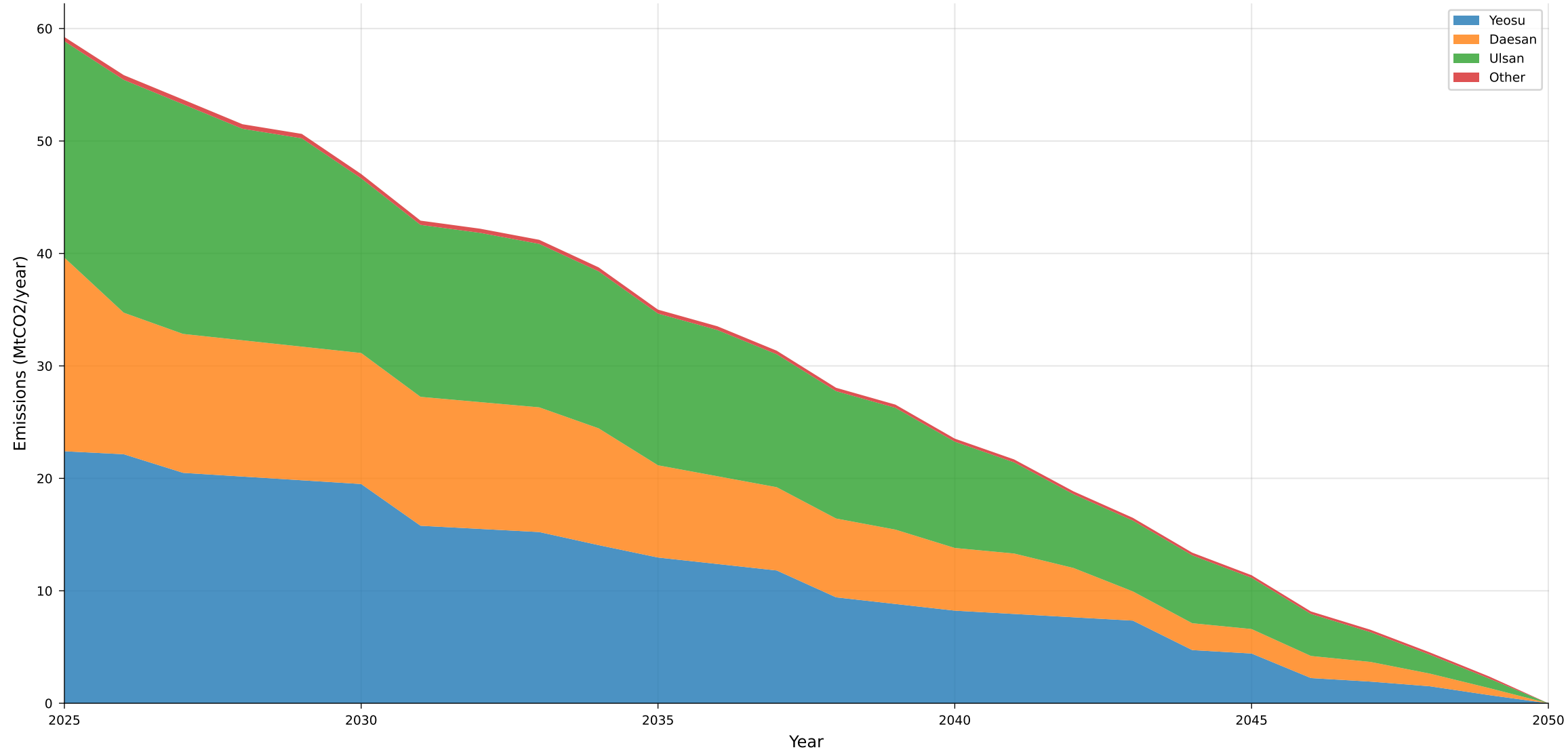
Emission Pathway by Region - NCC-H2 (Rising + Decoupled)
