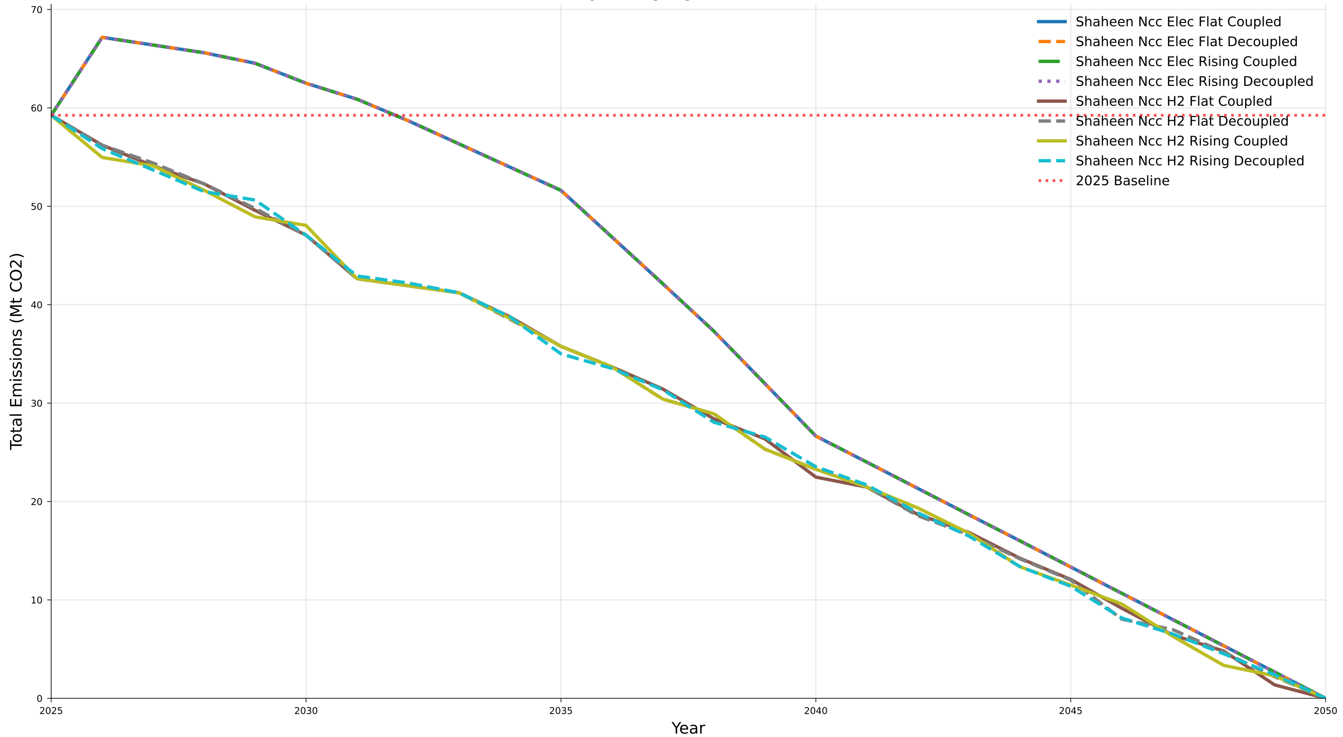
Emissions Trajectory by Scenario (2025-2050)
