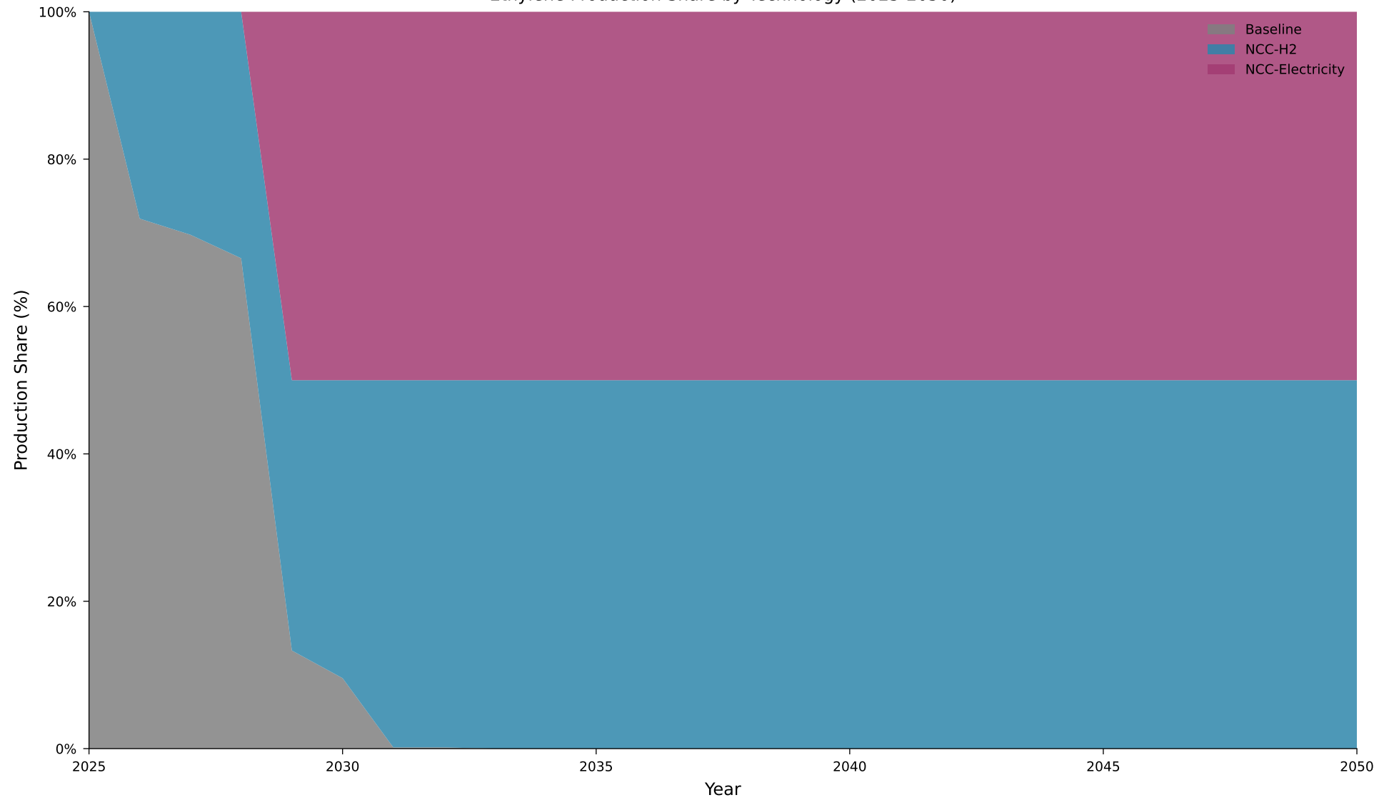
Ethylene Production Share by Technology (2025-2050)
