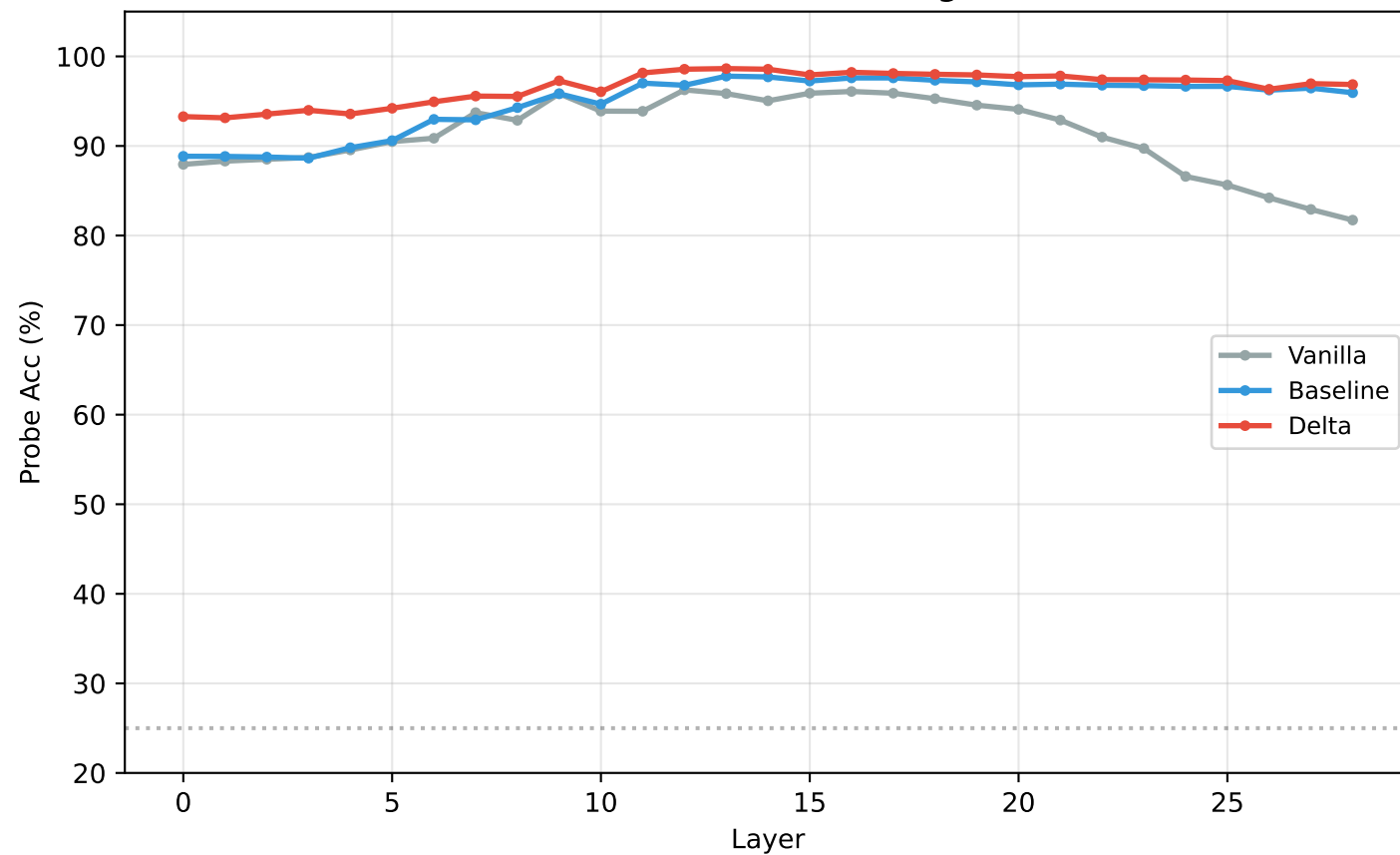
Answer Token — in-task (diagonal)
