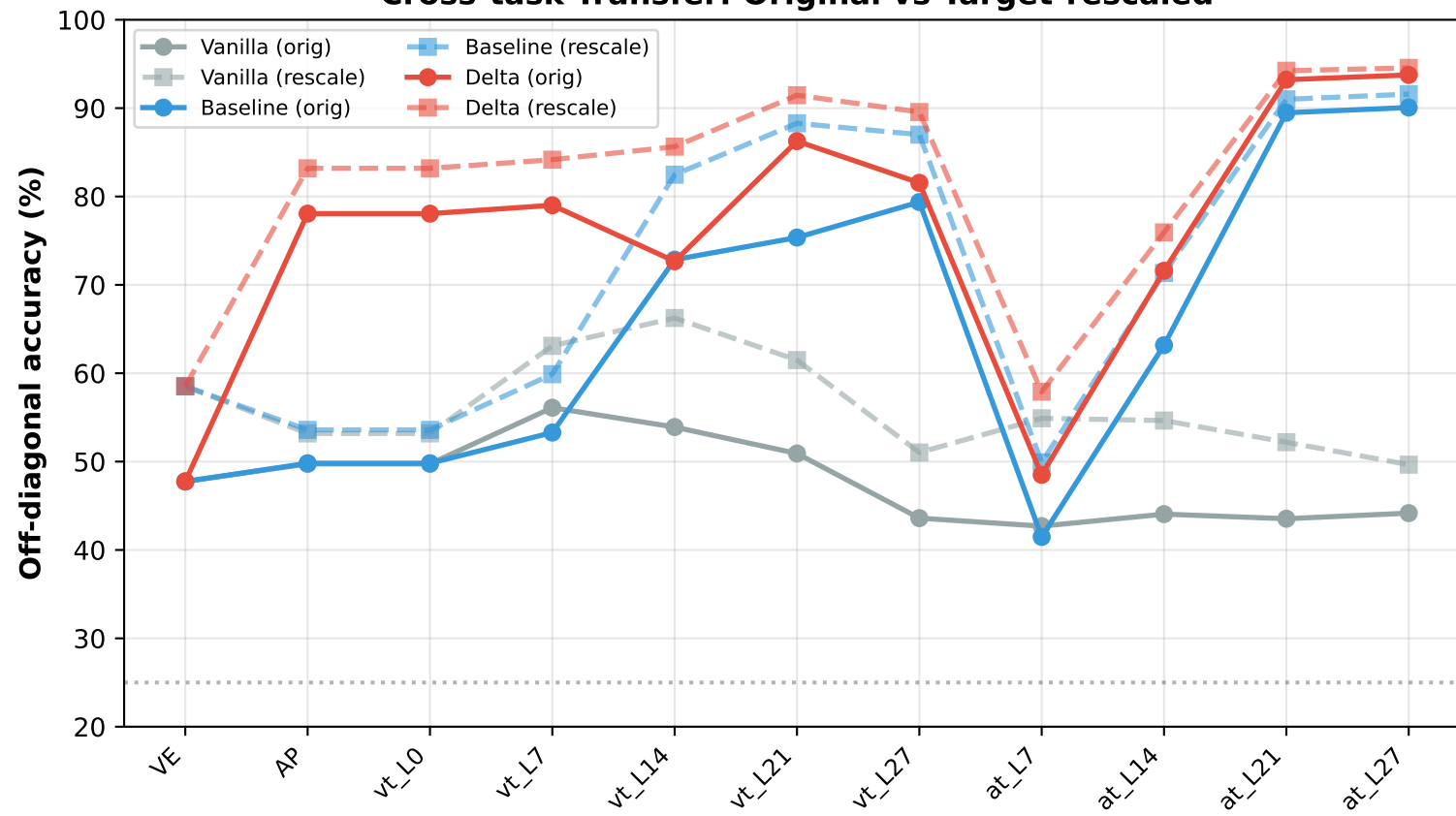
Cross-task Transfer: Original vs Target-rescaled
