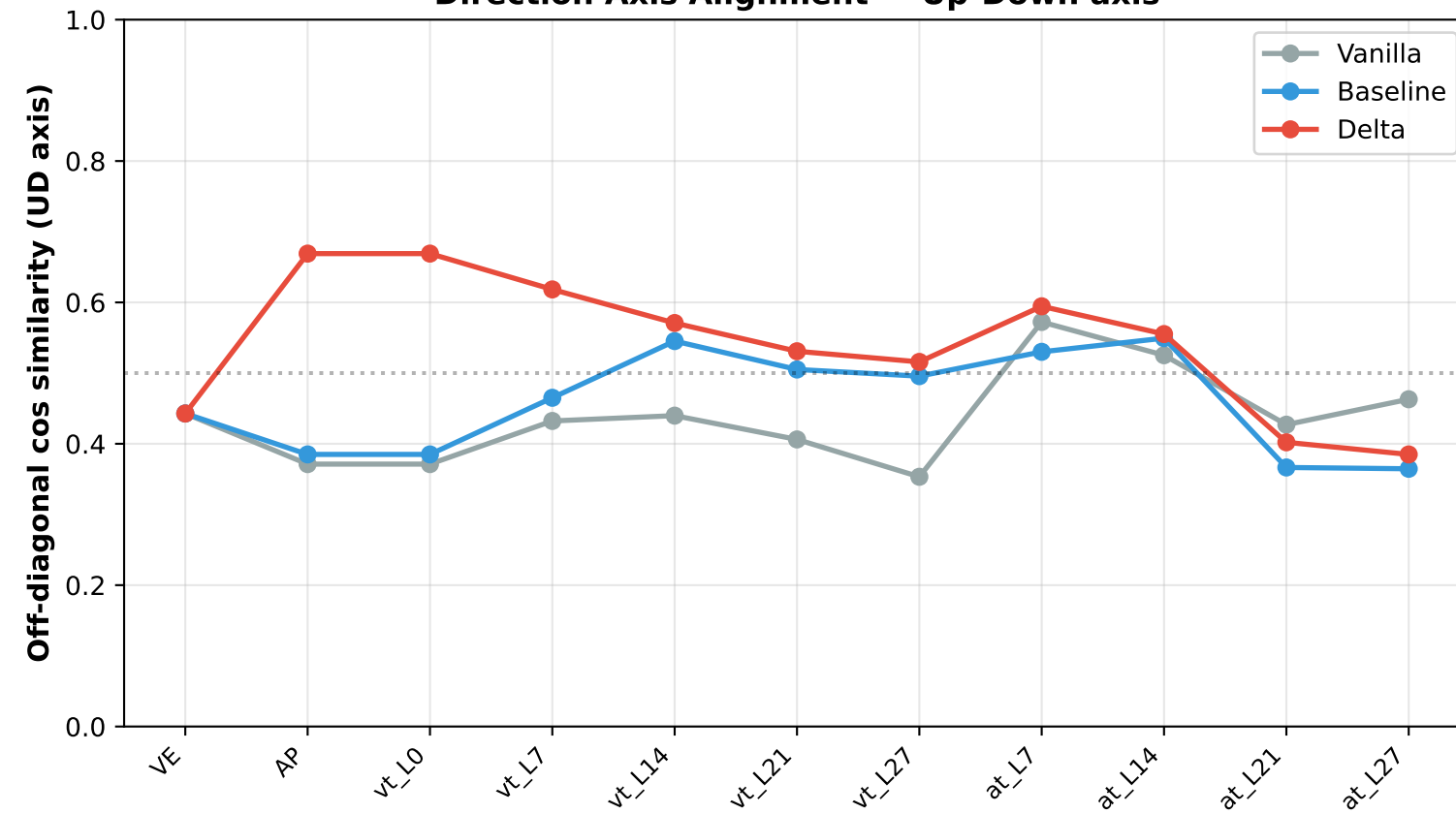
Direction Axis Alignment — Up-Down axis
