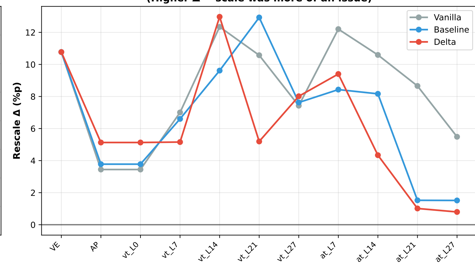
Scale Contribution to Cross-task Gap (Higher \Delta = scale was more of an issue)
