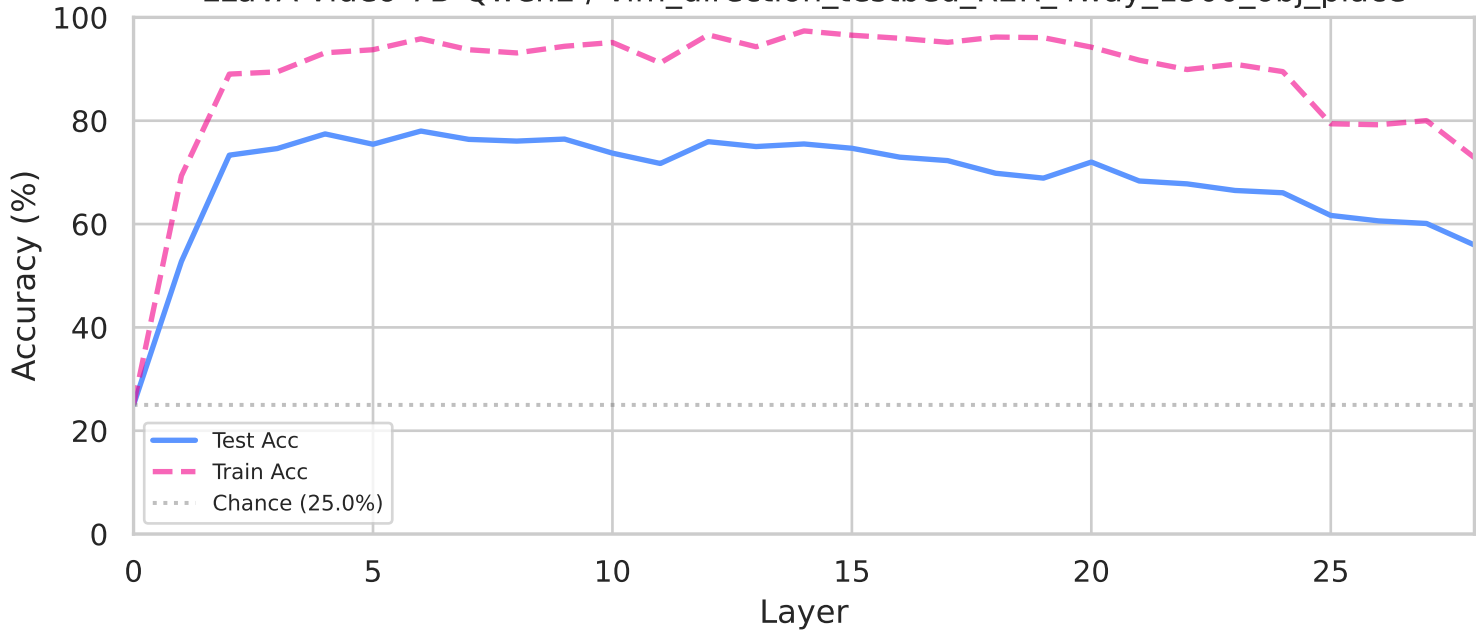
Linear Probing per Layer LLaVA-Video-7B-Qwen2 / vlm_direction_testbed_R2R_4way_1500_obj_place
