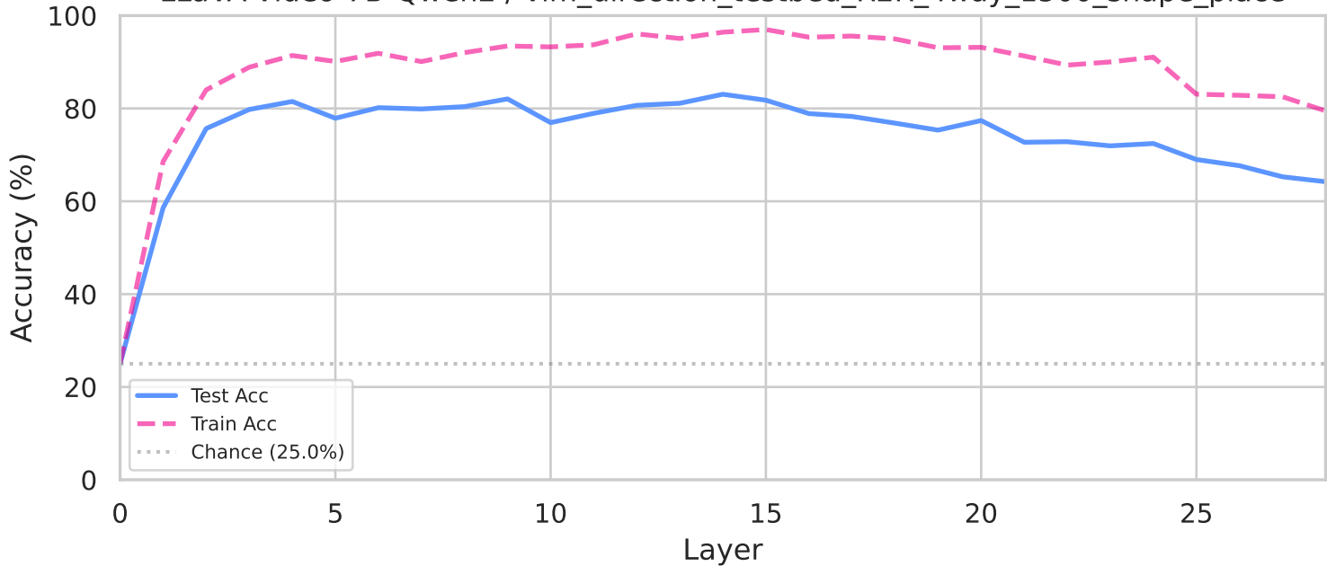
Linear Probing per Layer LLaVA-Video-7B-Qwen2 / vlm_direction_testbed_R2R_4way_1500_shape_place
