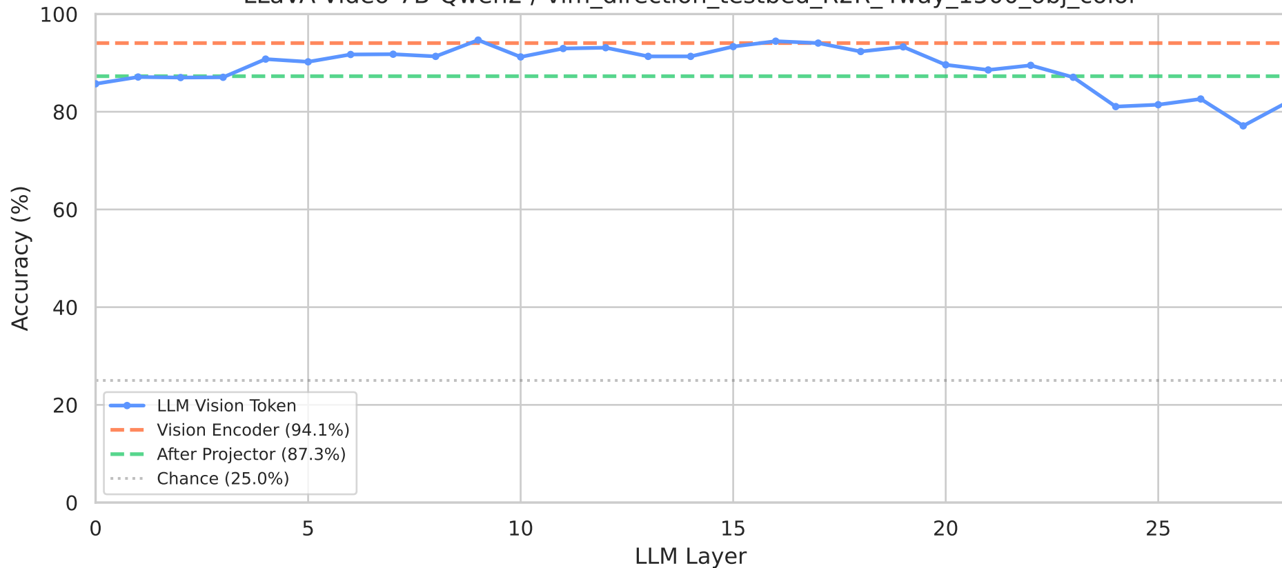
Linear Probing: Vision Information Flow LLaVA-Video-7B-Qwen2 / vlm_direction_testbed_R2R_4way_1500_obj_color
