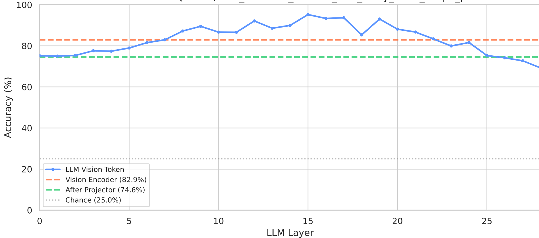
Linear Probing: Vision Information Flow LLaVA-Video-7B-Qwen2 / vlm_direction_testbed_R2R_4way_1500_shape_place
