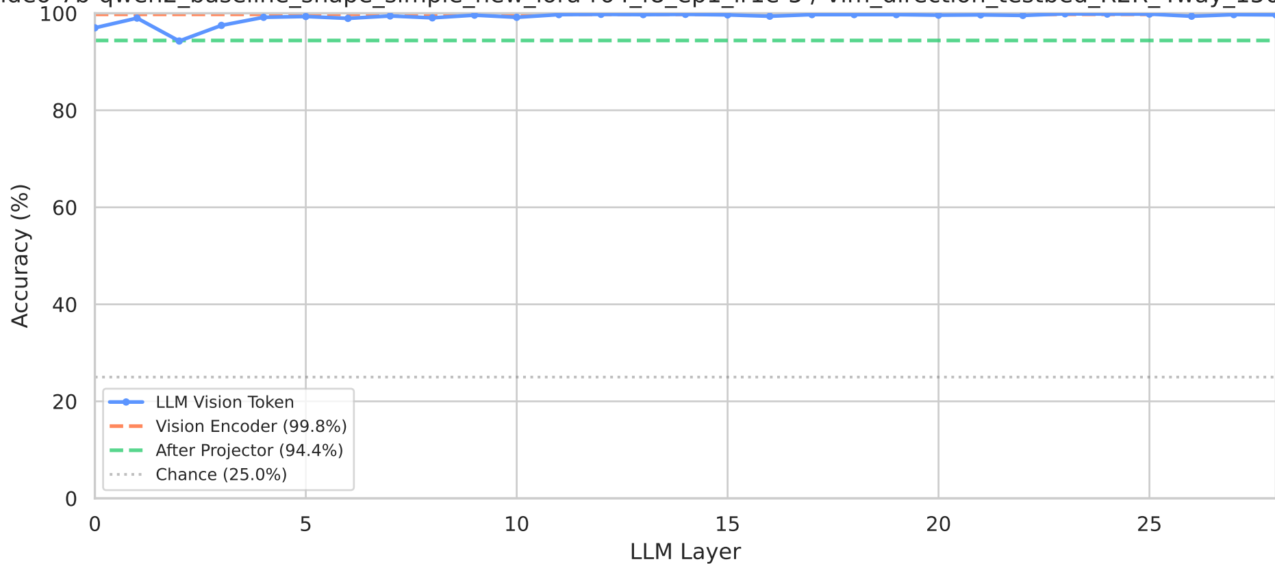
Linear Probing: Vision Information Flow video-7b-qwen2_baseline_shape_simple_new_lora-r64_f8_ep1_lr1e-5 / vlm_direction_testbed_R2R_4way_1500
