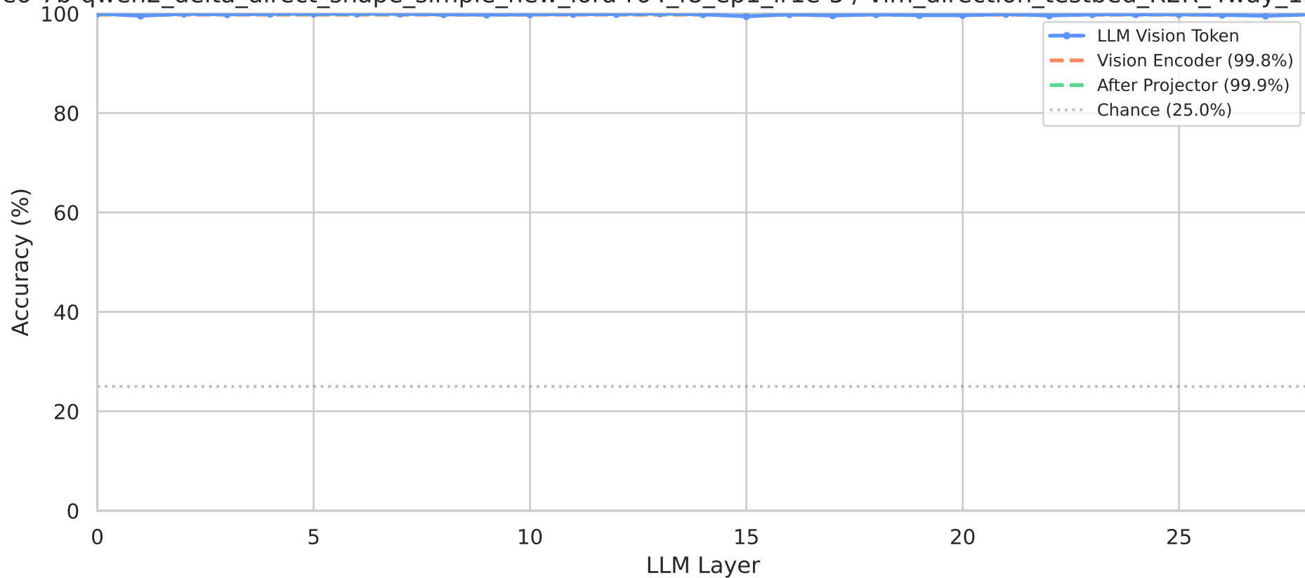
Linear Probing: Vision Information Flow deeo-7b-qwen2_delta_direct_shape_simple_new_lora-r64_f8_ep1_lr1e-5 / vlm_direction_testbed_R2R_4way_150
