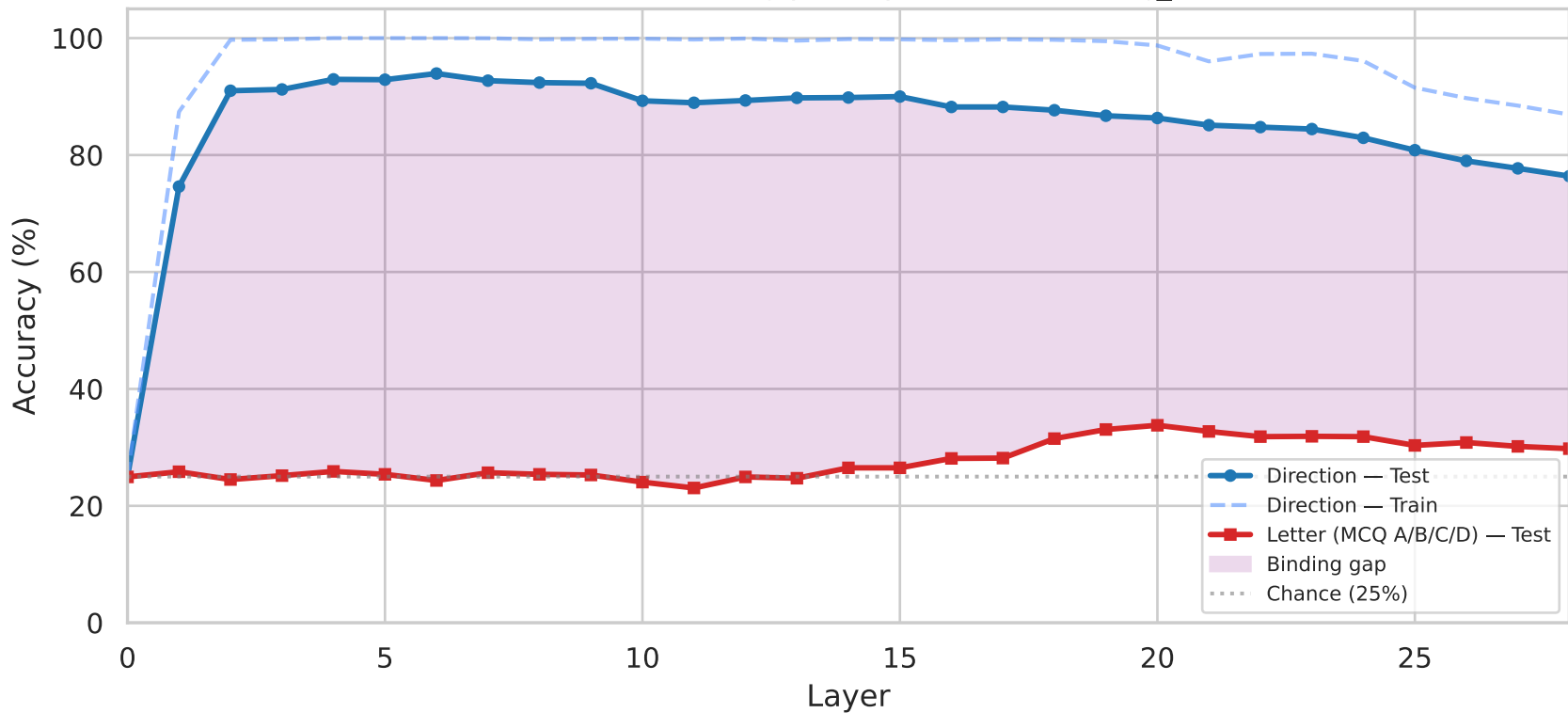
Answer Token Probing per Layer — Vanilla / obj_color
