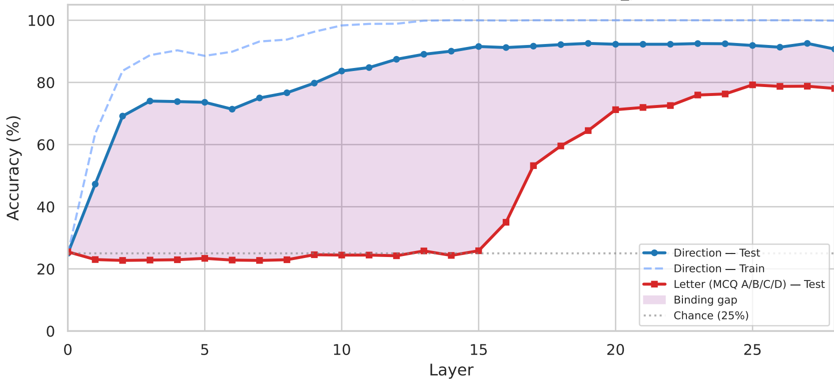
Answer Token Probing per Layer — Baseline / obj_place
