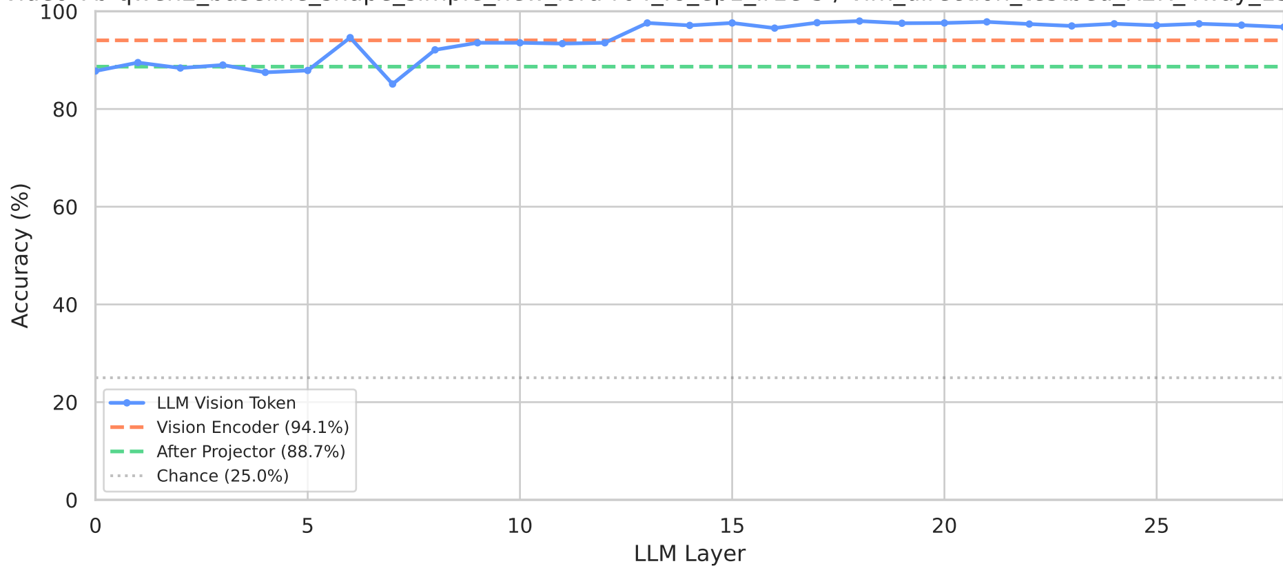
Linear Probing: Vision Information Flow a-video-7b-qwen2_baseline_shape_simple_new_lora-r64_f8_ep1_lr1e-5 / vlm_direction_testbed_R2R_4way_150
