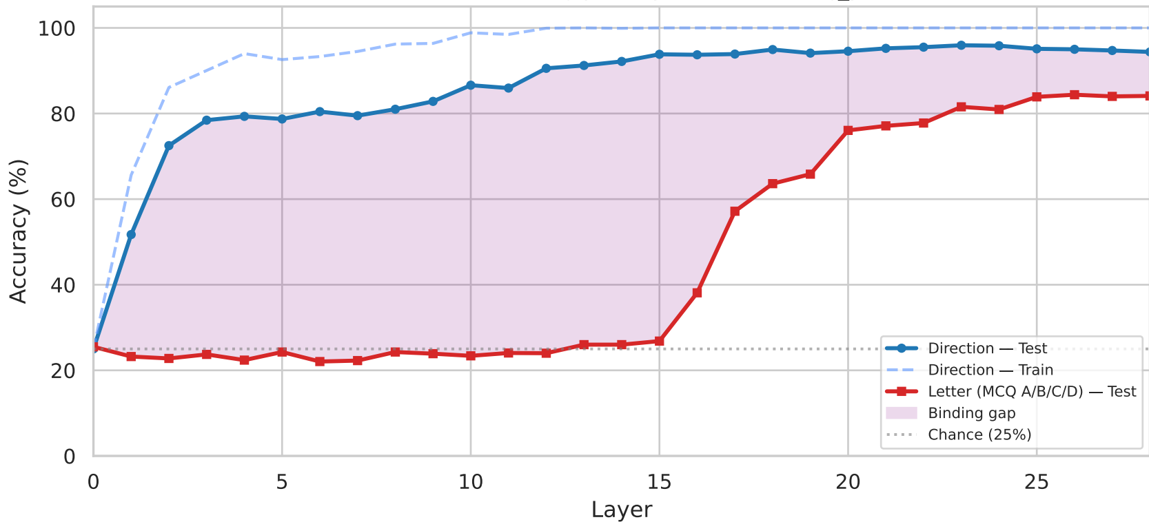
Answer Token Probing per Layer — Delta / obj_place
