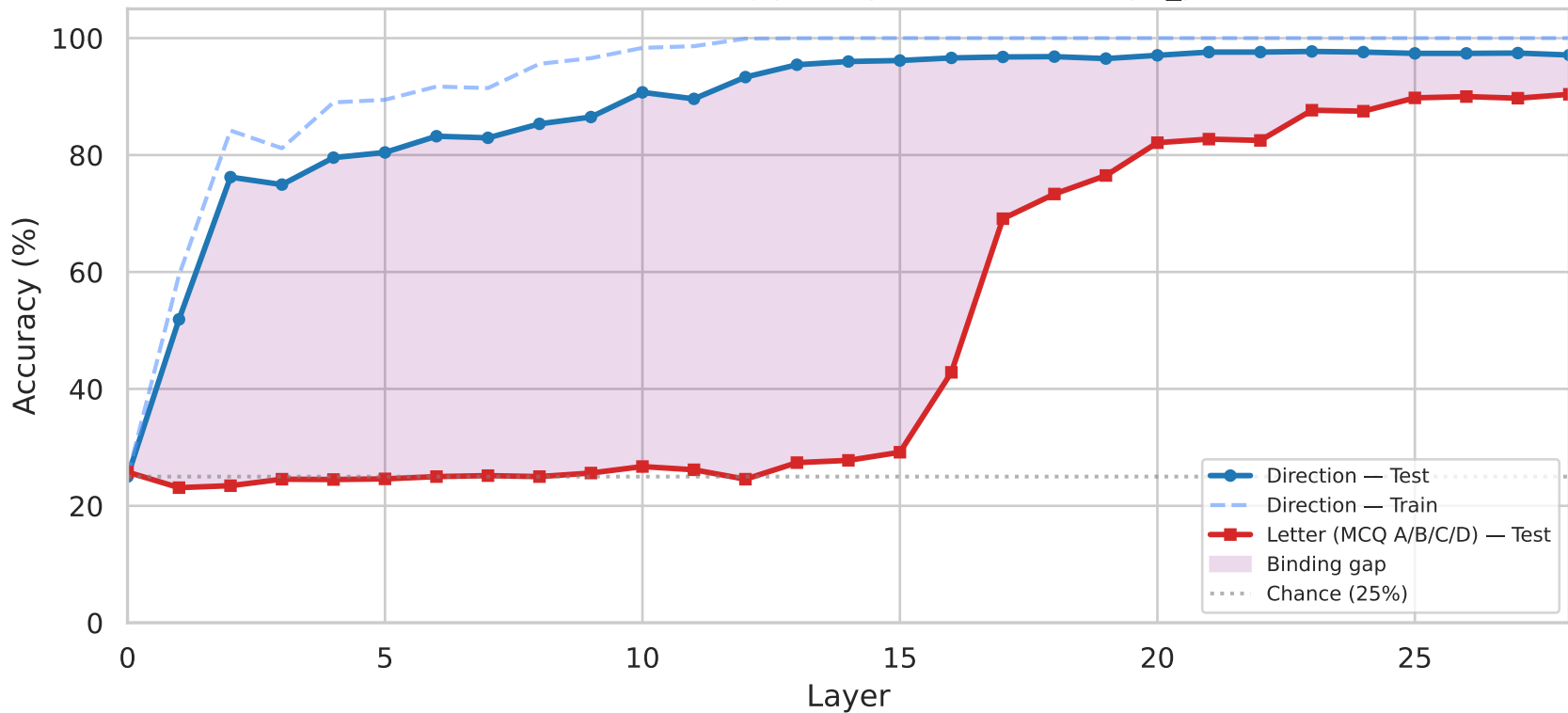
Answer Token Probing per Layer — Delta / shape_place
