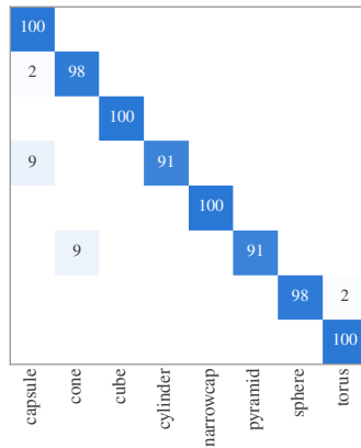
Moving, occluded acc 97.4% (n=386)
