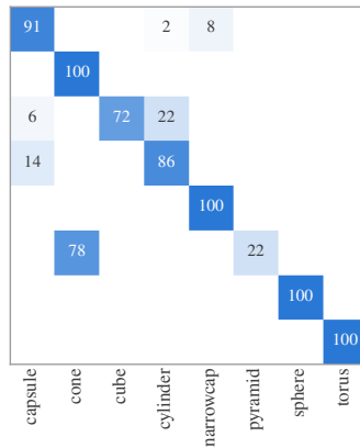
Static, occluded acc 82.7% (n=393)
