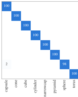
Moving, no occluder acc 99.7% (n=390)
